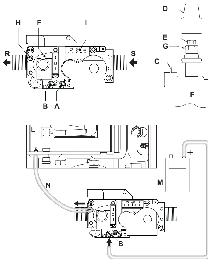
fig. 29 - Valvola gas
